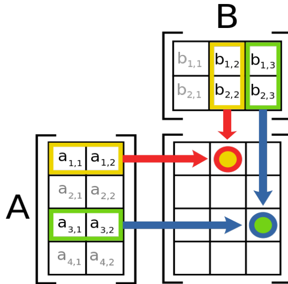
Figure 1: Matrix multiplication
